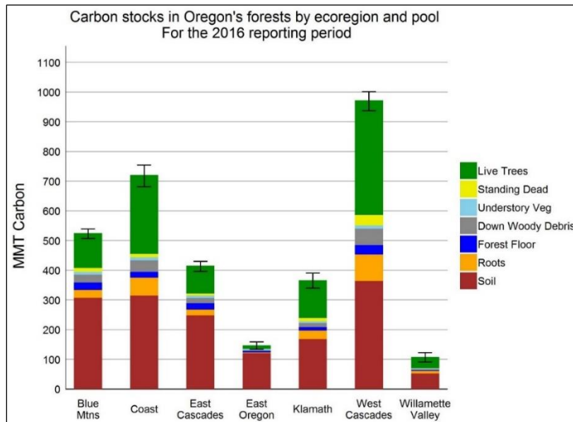
Figure 2.4: Average carbon stock (MMT C) by pool and ecological region, 2007-16. Error bars represent a 95% confidence interval of estimated total stock for each region (Christensen et al. 2019).
