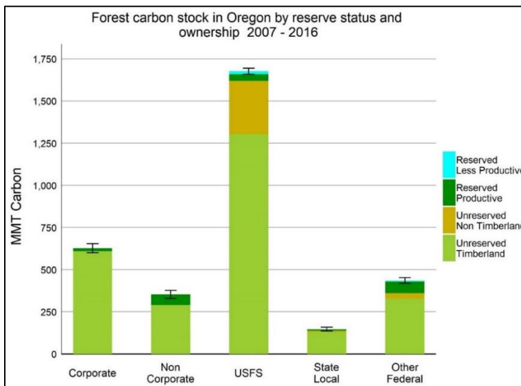
Figure 2.3: Oregon statewide average forest carbon stock by reserve status and ownership, 2007-16 (MMT). Error bars represent 95% confidence interval of estimated total stock for each ownership (Christensen et al. 2019).
