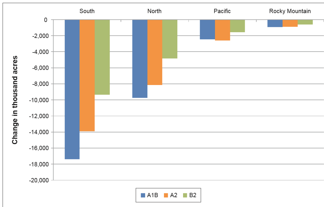
Figure 3.3: Change in conterminous U.S. nonfederal forest area from 2010-60 by RPA assessment region and RPA scenario (thousand acres) (USFS 2012).
