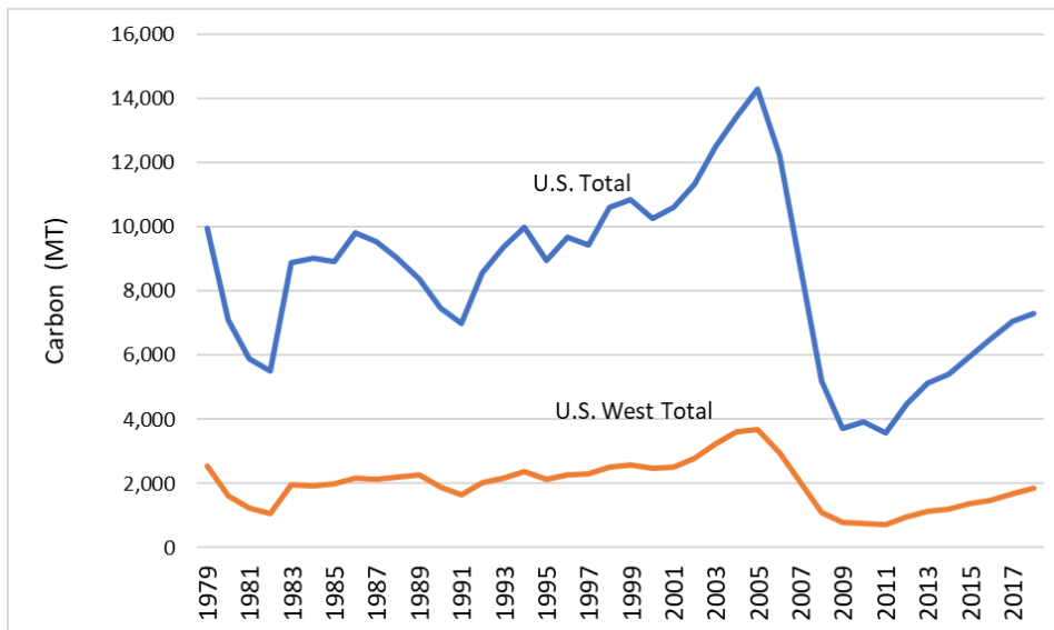
Figure 4.3: Annual new carbon storage in the United States (blue line) and in the western United States (orange line) for single-family housing stock (U.S. Census 2019).
