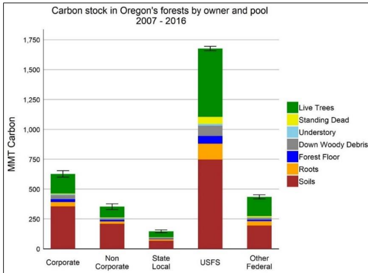
Figure 2.2: Oregon statewide average forest carbon stock by pool and ownership, 2007-16 (MMT). Error bars represent a 95% confidence interval of estimated total stock for each ownership (Christensen et al. 2019).
