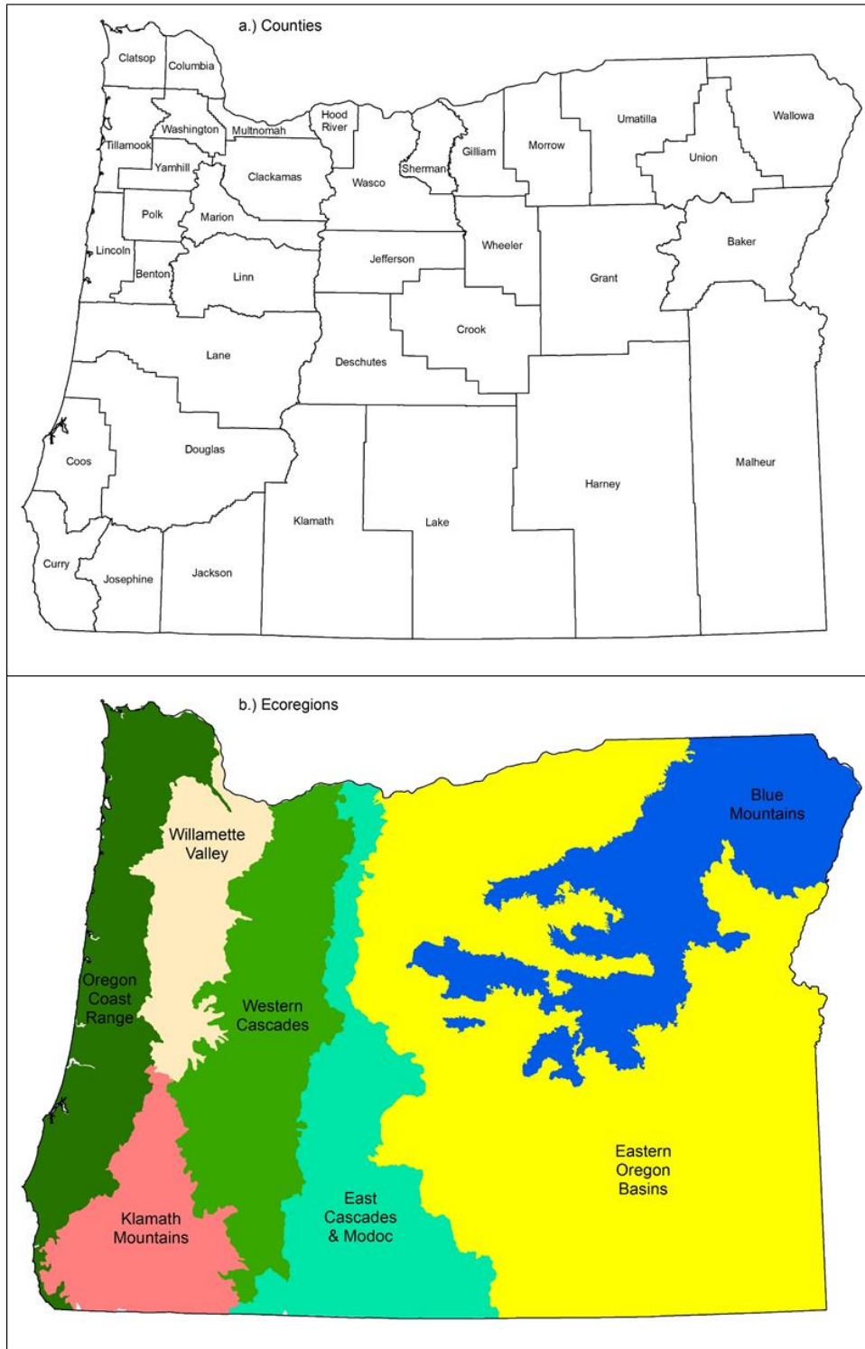
Figure 2.8: Oregon a.) counties and b.) ecoregions, based on ecological sections as described by Cleland et al. (2007) (Christensen et al. 2019).
