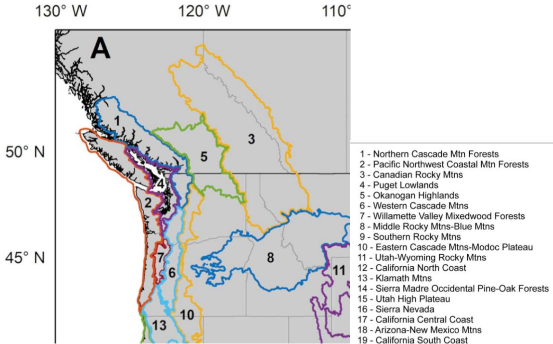
Figure 3.5: Climatic ecoregions in the Pacific Northwest (Hessburg et al. 2019).
