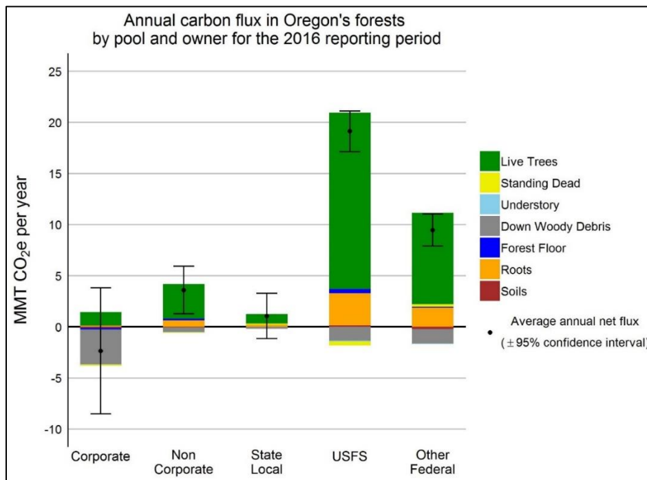
Figure 2.6: Oregon statewide estimate of average annual carbon flux (MMT CO 2 e/year) by pool and ownership, 2001-06 to 2011-16. Estimates exclude emissions from land-use changes and non-CO 2 greenhouse gases. Roots includes belowground live and dead tree roots. Understory includes aboveground and belowground pools. Error bars represent 95% confidence intervals around point estimates for net flux (Christensen et al. 2019).
