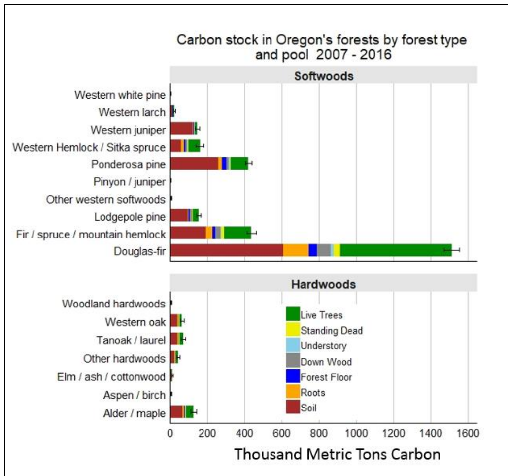
Figure 2.5: Oregon statewide average carbon stock by pool and forest type, 2007-16 (thousand metric tons C). Error bars represent a 95% confidence interval of total stock for each forest type (Christensen et al. 2019).
