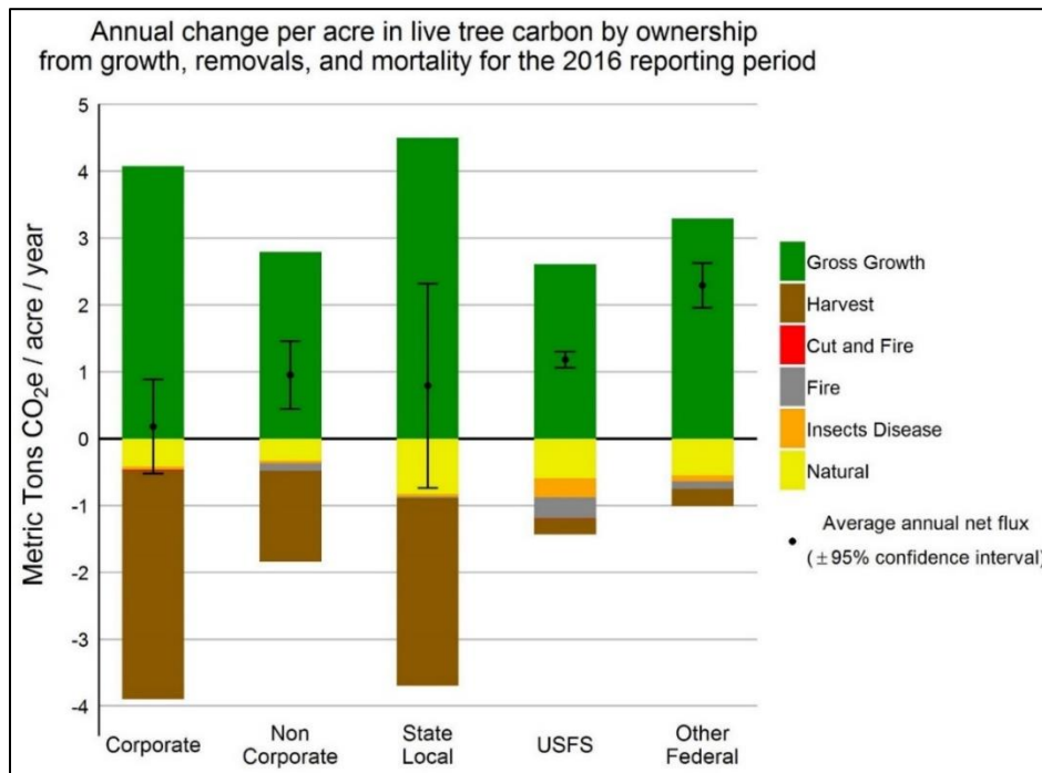
Figure 2.7: Average annual net change per acre in aboveground live tree carbon (MT/CO 2 e/acre) by ownership in Oregon’s forests, 2001-06 to 2011-16. The error bars represent a 95% confidence interval of net change (Christensen et al. 2019).
