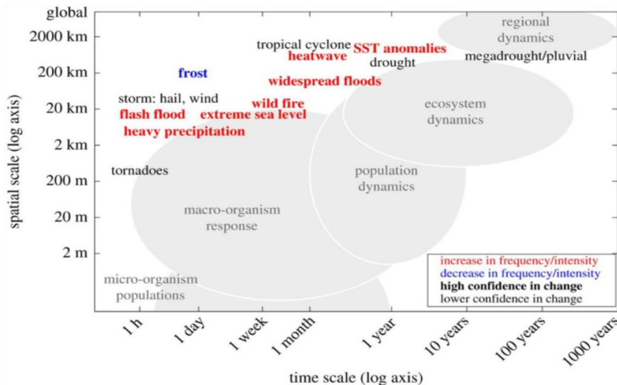
Figure 3.4: Spatial and temporal scales of typical extreme weather and climate events and the biological systems they impact (IPCC 2019).
