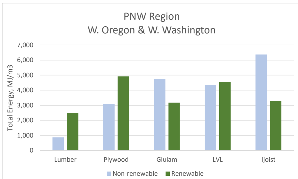
Figure 4.11: Total energy (A1-A3) use for selected wood products produced in the PNW (from 2012 production surveys: www.corrим.org/latest-reports/ ).
