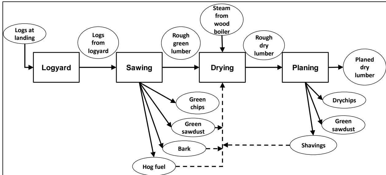
Figure 4.10: Diagram of the relationships between processes used to create PNW planed dry lumber from logs. Dotted line indicates that a portion of the product is burned at the dryer. (Milota 2015, 2020).
