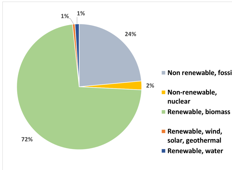
Figure 4.12: Average representation of fuel source for total energy demand for production of softwood lumber in the PNW (Milota 2015, 2020).
