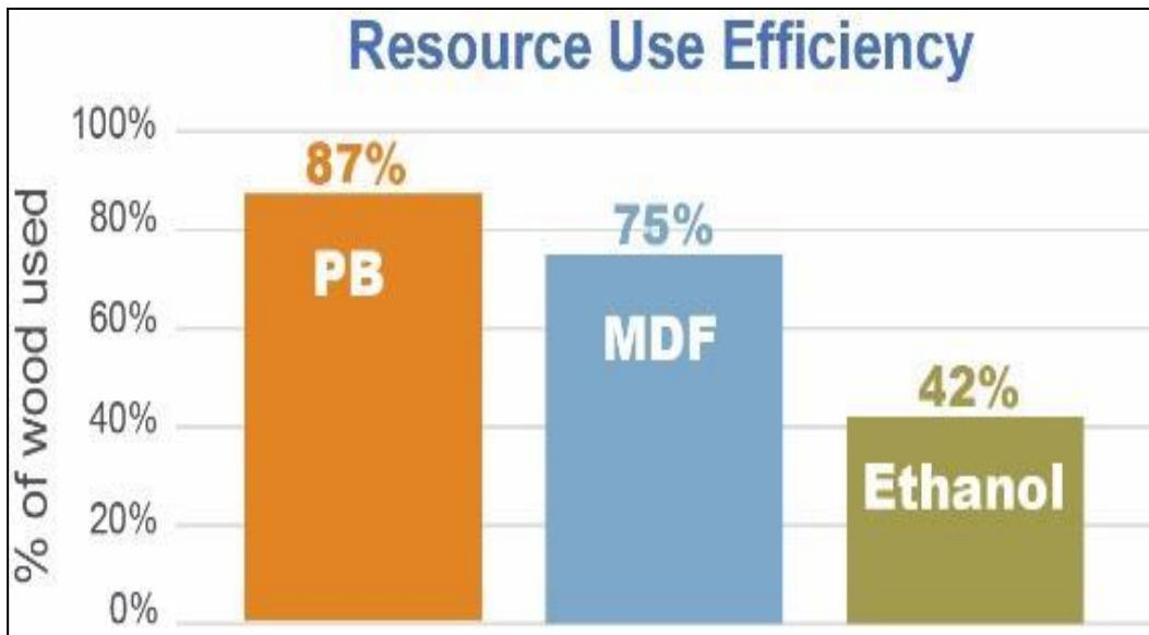
Figure 4.13: Percent wood used in final product, or resource use efficiency, for wood residues used for producing particleboard (PB), medium-density fiberboard (MDF) and ethanol.
