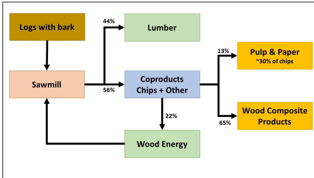
Figure 4.4: Flow material in an average PNW softwood lumber production facility (data is based on surveys of manufacturers located in Oregon and Washington in 2012; Milota 2015, Puettmann 2019).
