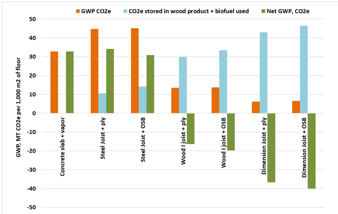
Figure 4.8: Cradle-to-gate (A1-A3) GWP for different structural assemblies in 1,000 square meters of floor area (Lippke et al. 2019).
