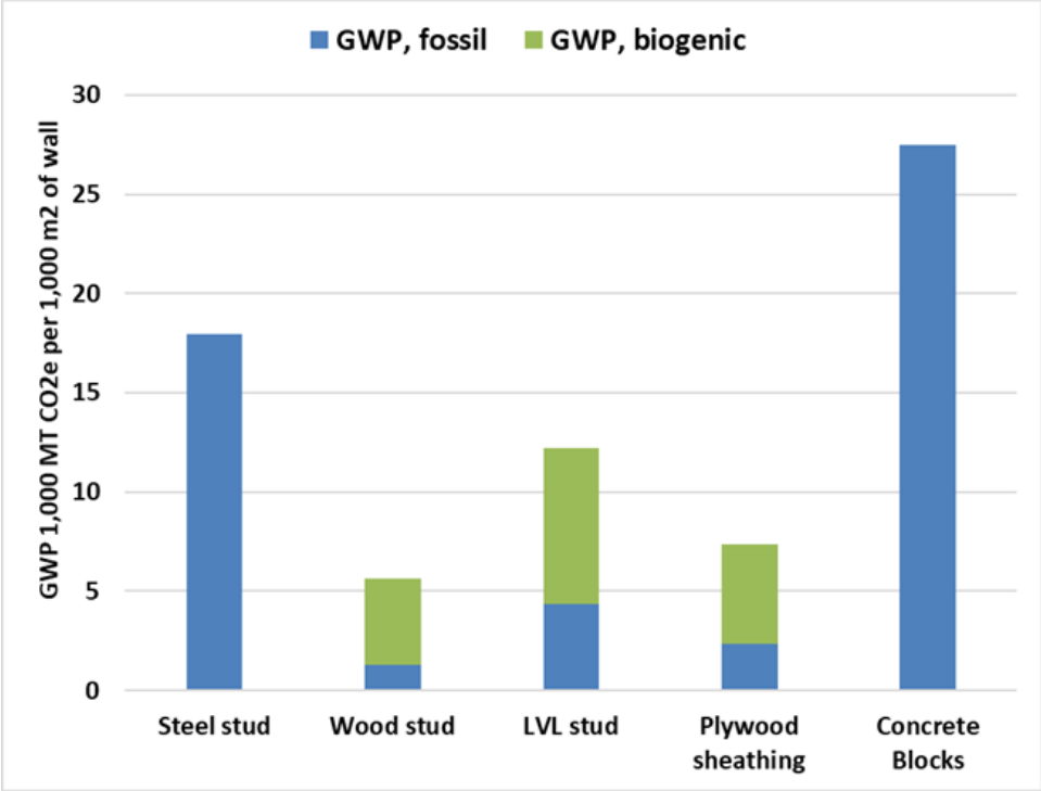
Figure 4.7: Cradle-to-gate (A1-A3) GWP for different structural components in a 1,000-square-meter wall. No hardware, insulation, gypsum, etc., is included. GWP biogenic emission includes carbon emissions from slash burning for more effective forest regeneration. (Lippke et al. 2019).
